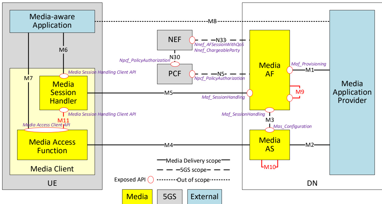
Figure 5 3GPP Media Delivery Architecture – Session Handling and Media Delivery
